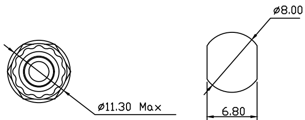
PANEL MOUNT
