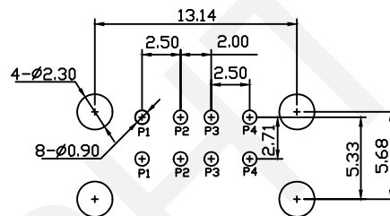
RECOMMENDED PCB PATTERN LAYOUT
